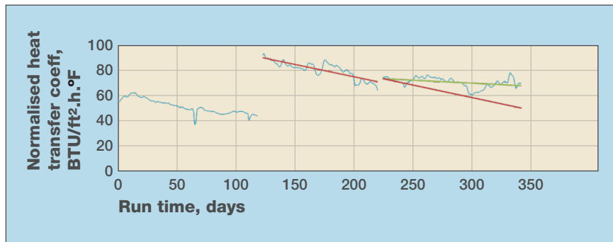
Figure 2 Improved heat transfer on exchanger bundle 2
