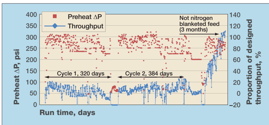
Figure 4 Rapid fouling because the storage tank was not nitrogen blanketed
