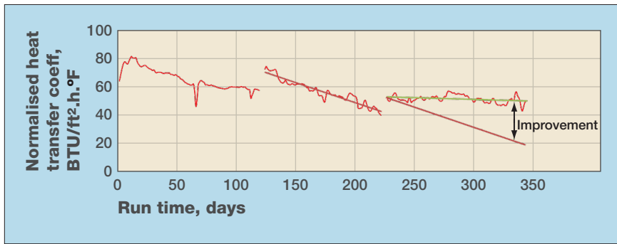
Figure 1 Improved heat transfer on exchanger bundle 1
