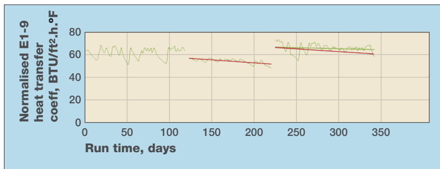
Figure 3 Improved heat transfer on exchanger bundle 4
