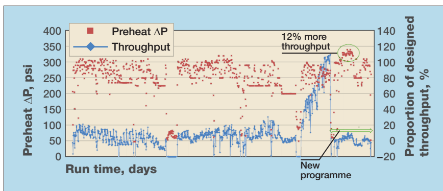
Figure 5 Lower pressure drop and increased throughput
